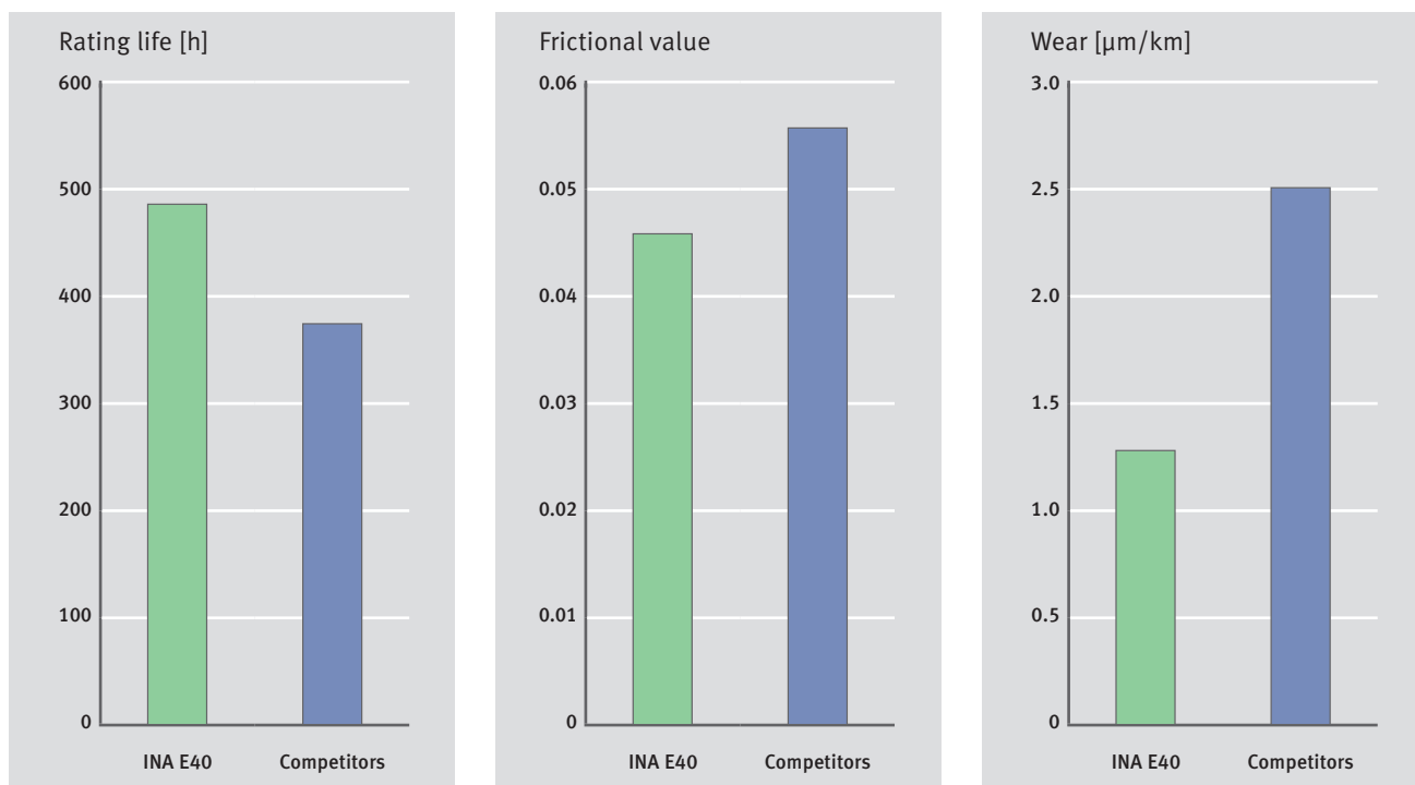
The test results are based on the following test conditions: P = 80 kN, p = 50 N/mm 2 , β = 60°, f = 43.3 min -1 , v = 30.25 mm/s
